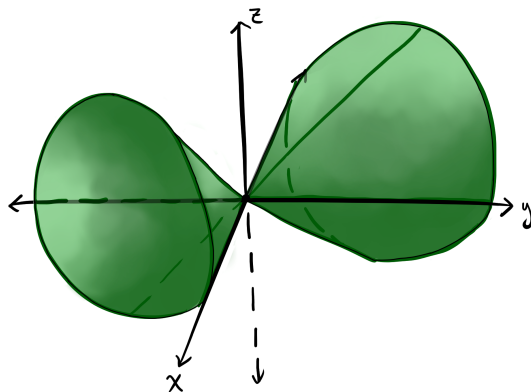
Figure 1.3: The vanishing locus V(xy - z^2) inside \mathbb{A}^3
